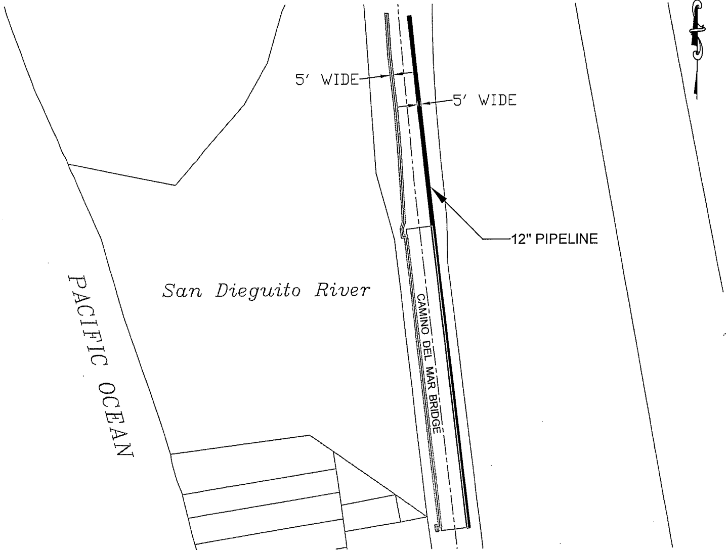
12" GAS PIPELINE CAMINO DEL MAR BRIDGE, SAN DIEGUITO RIVER
