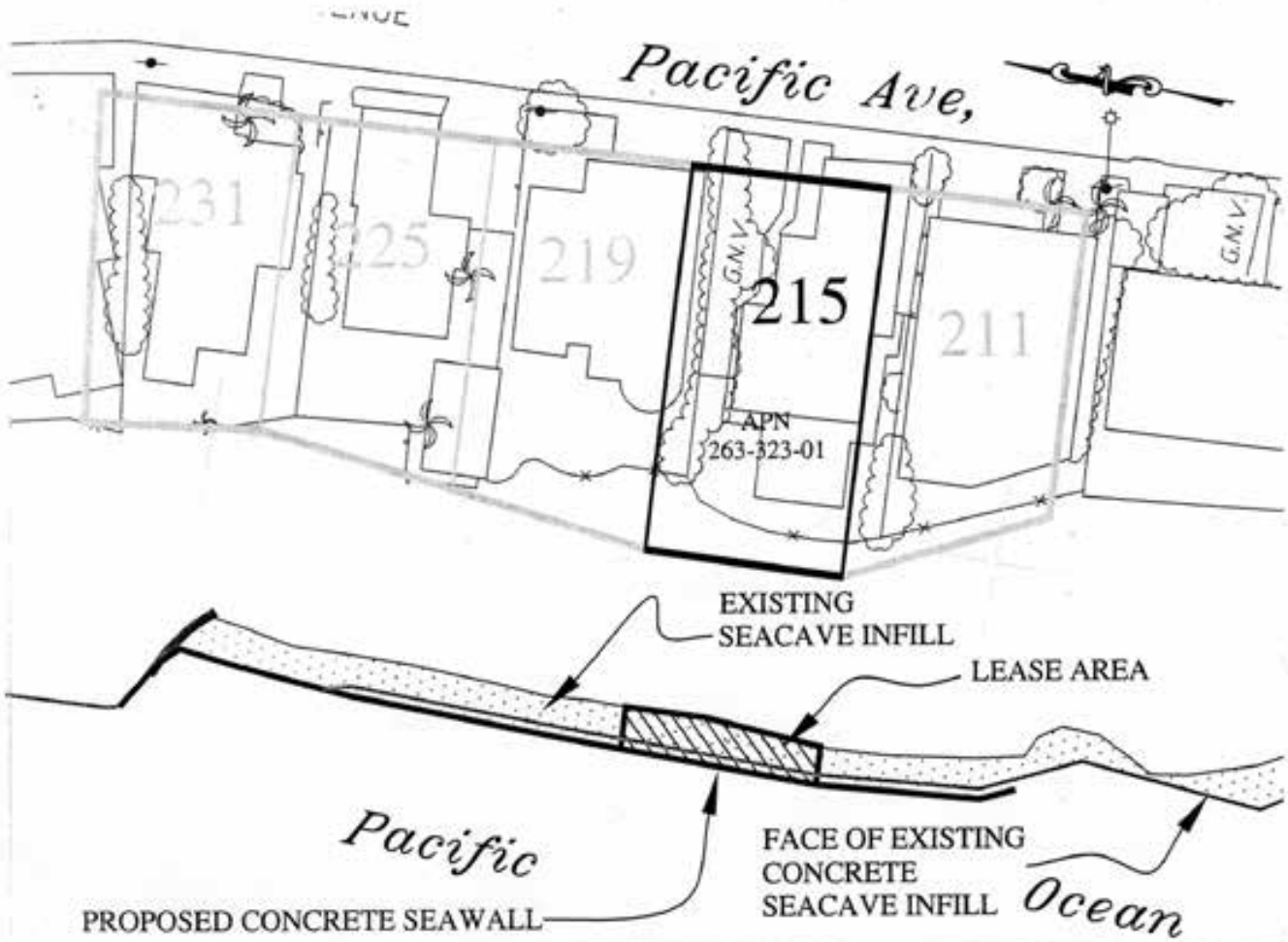
215 PACIFIC AVENUE, SOLANA BEACH PROPOSED SEAWALL AND EXISTING SEA CAVE INFILL
