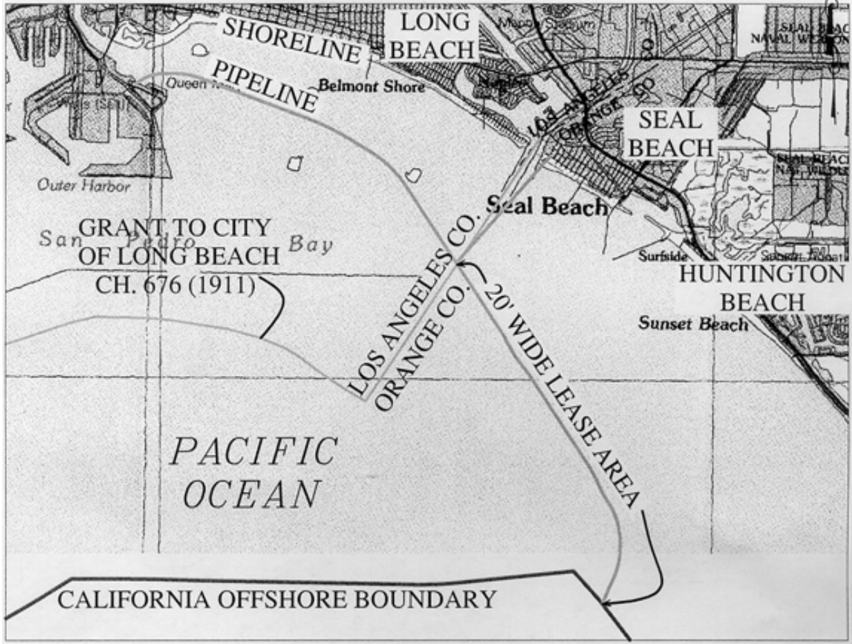
Existing 16" Diameter Crude Oil Pipeline Offshore of the Cities of Seal Beach and Huntington Beach
