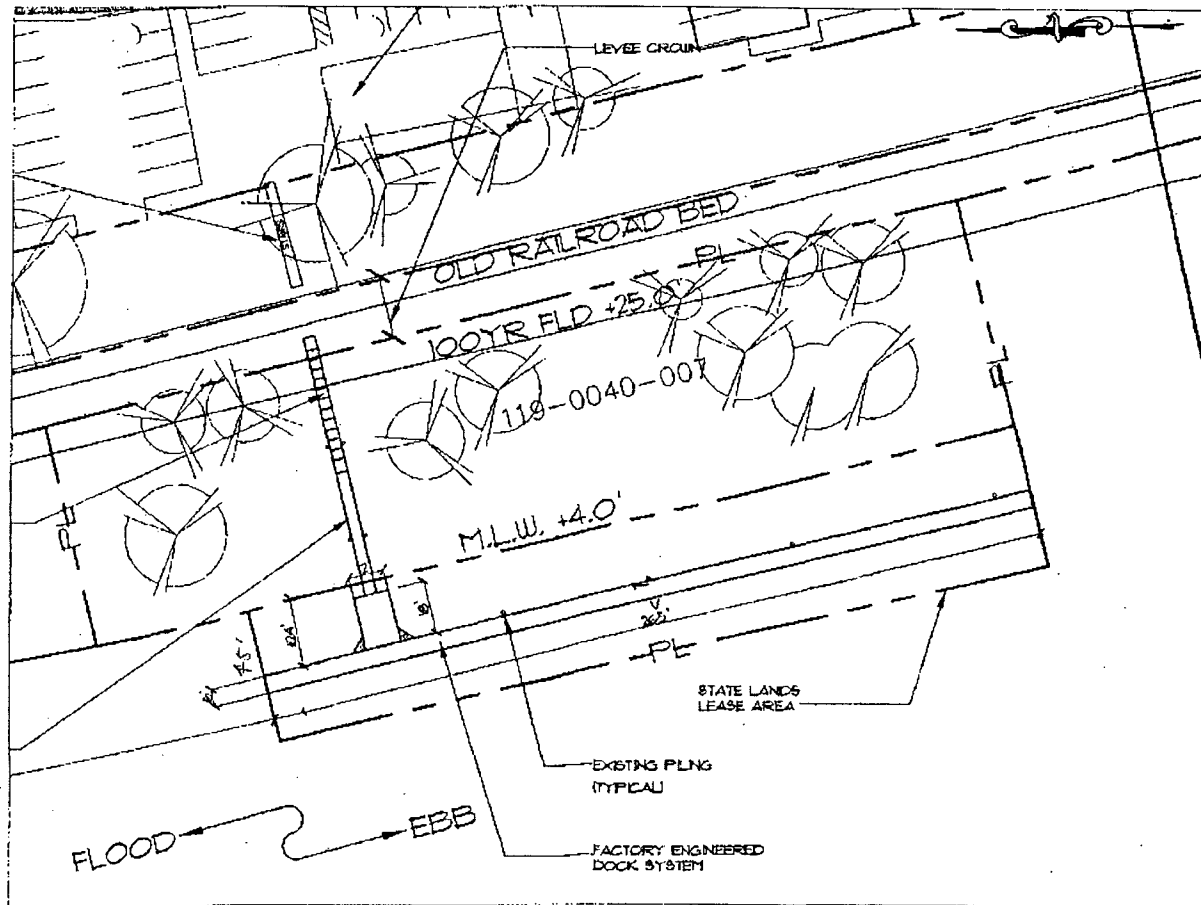
SACRAMENTO RIVER AT FREEPORT
