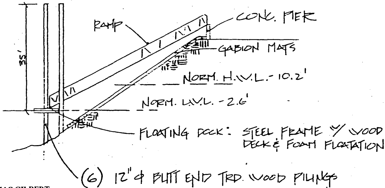
SIDE ELEVATION 1" = 20'
