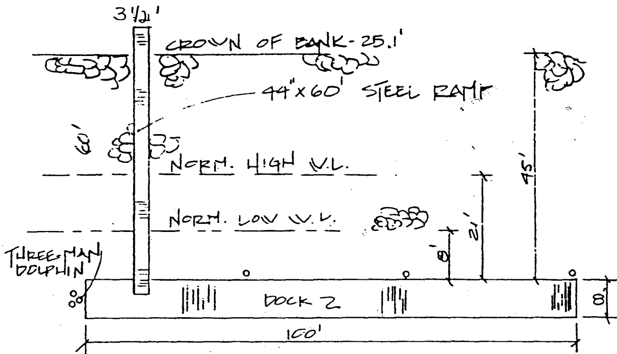
PLAN VIEW 1" = 20'
