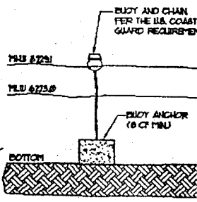
BUOY DETAIL NO SCALE
