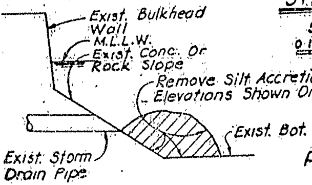
TYPICAL SECTION NO SCALE
